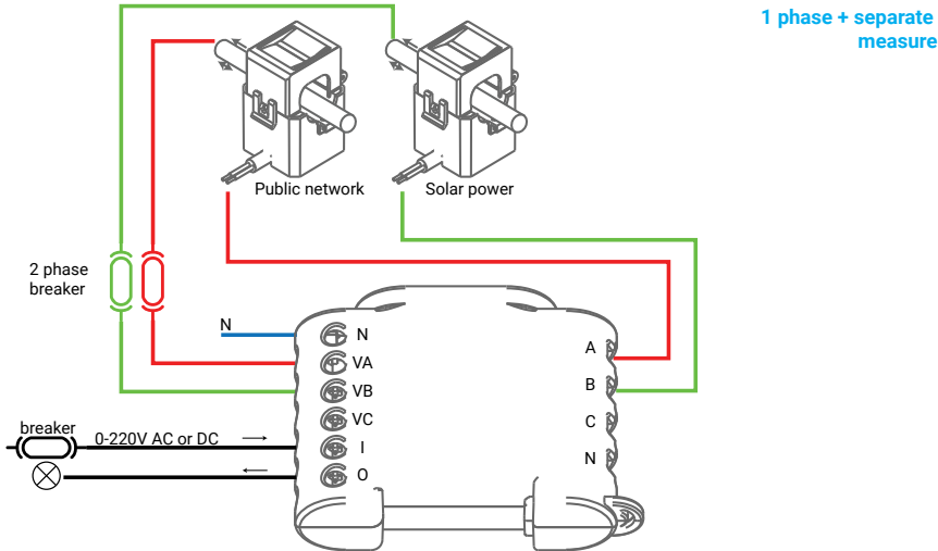
1 phase wiring up to 3 different circuits
