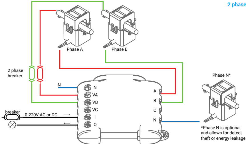
1 phase + separate solar power measurement wiring
